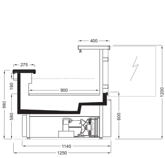
LEOPARD V1 900 WFG/SD
